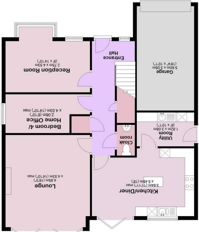
Ground Floor Approx. 103.9 sq. metres (1118.4 sq. feet)
