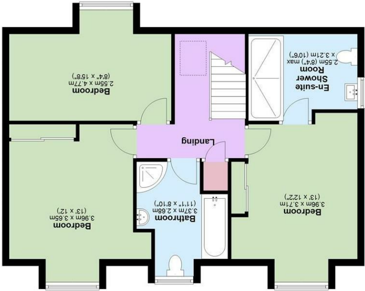
First Floor Approx. 71.3 sq. metres (767.8 sq. feet)
