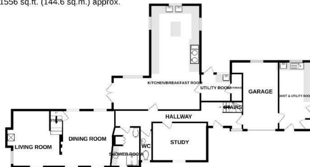
GROUND FLOOR 1556 sq.ft. (144.6 sq.m.) approx.
