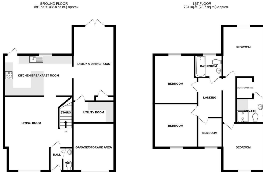
TOTAL FLOOR AREA: 1685 sq.ft. (156.6 sq.m.) approx. Made with Metropix ©2023
