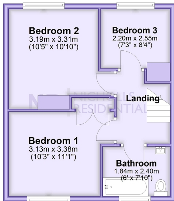
First Floor Approx. 41.0 sq. metres (440.8 sq. feet)
