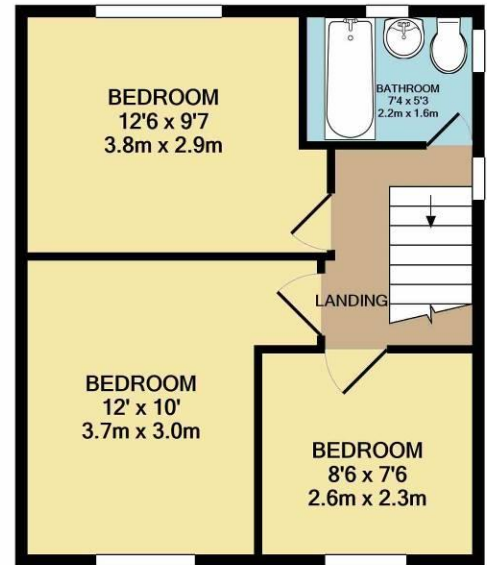
1ST FLOOR
