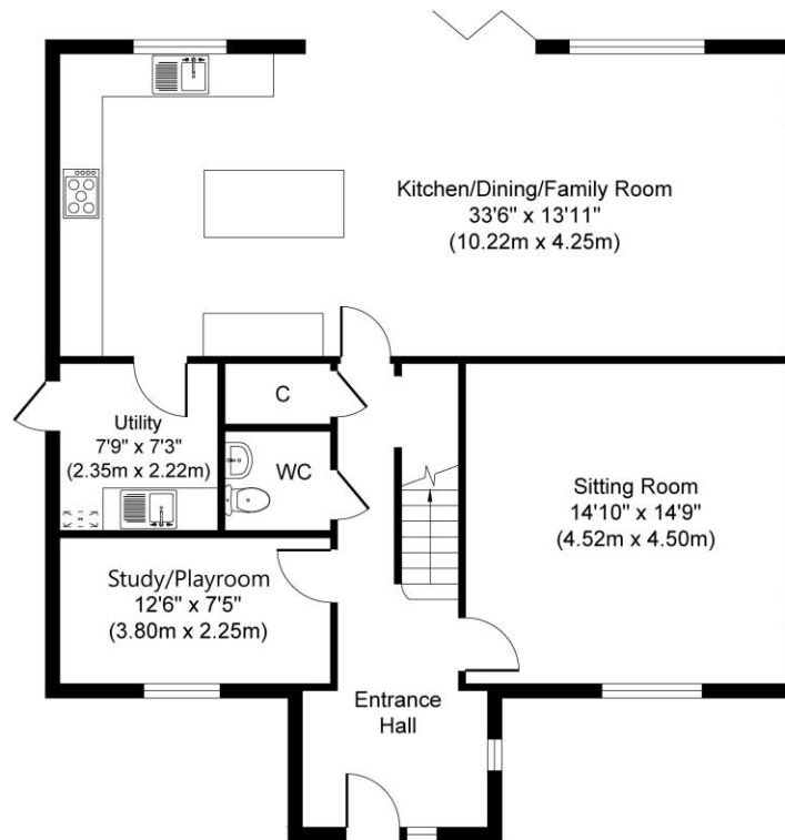
Ground Floor Approximate Floor Area 1,030 sq. ft (95.69 sq. m)
