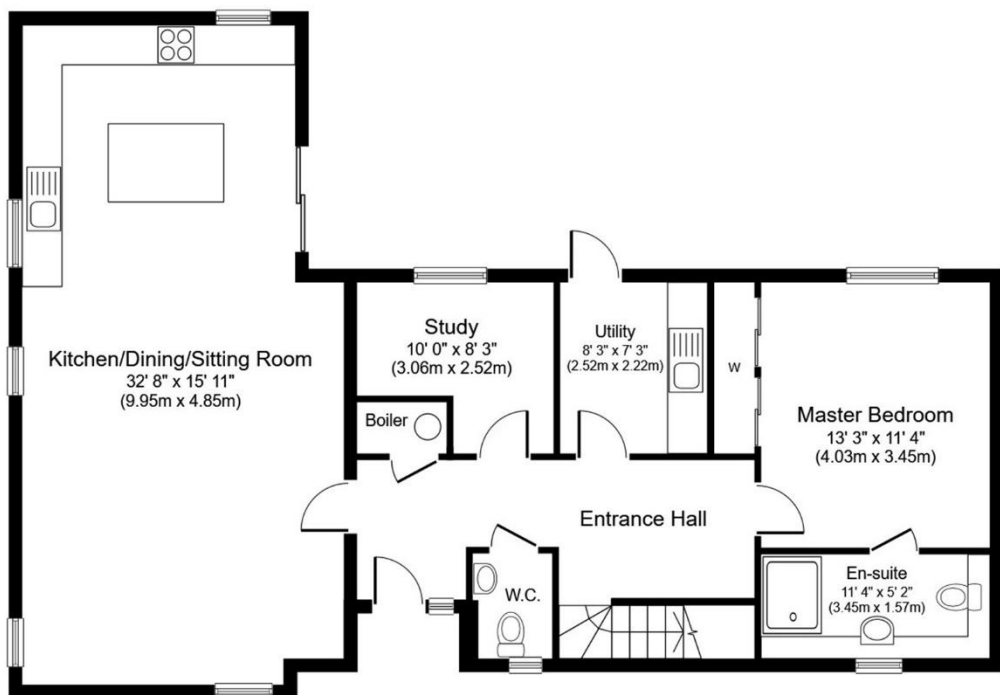
Ground Floor Approximate Floor Area 1,061 sq. ft. (98.6 sq. m.)
