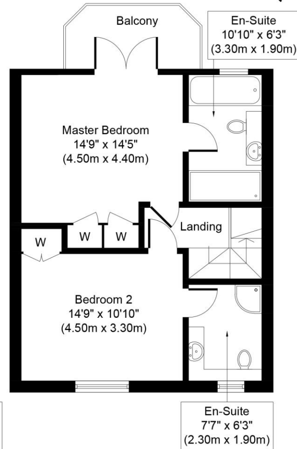
Second Floor Approximate Floor Area 535 Sq. ft. (49.7 Sq. m.)
