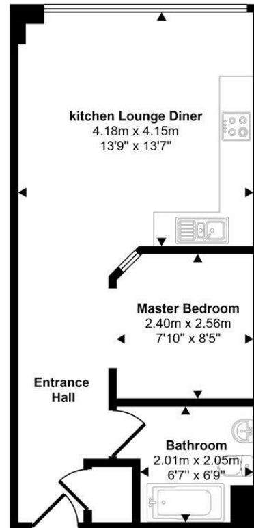
Floorplan
