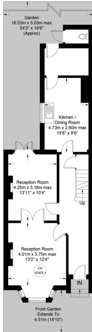
Ground Floor
