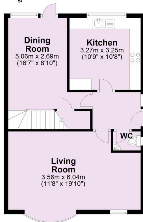
Ground Floor Approx. 52.6 sq. metres (566.3 sq. feet)
