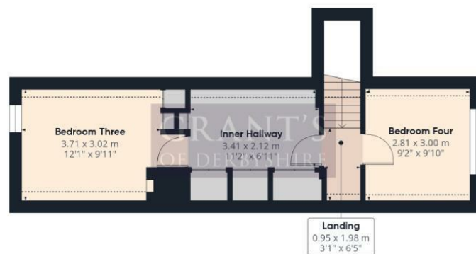
Floor 1 Building 1
