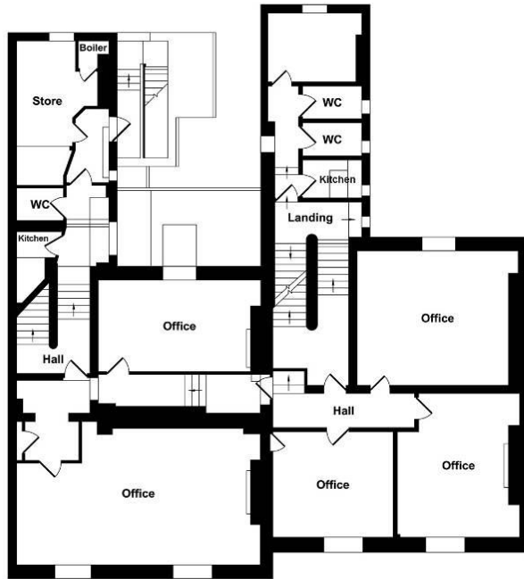
First Floor Offices
