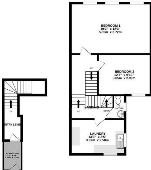
BUILDING FIRST FLOOR 689 sq.ft. (64.0 sq.m.) approx.
