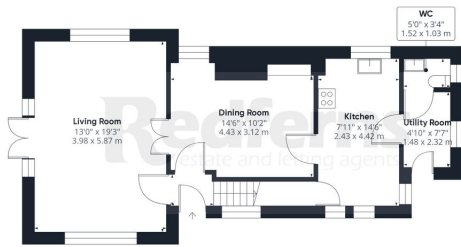
Floor 0
