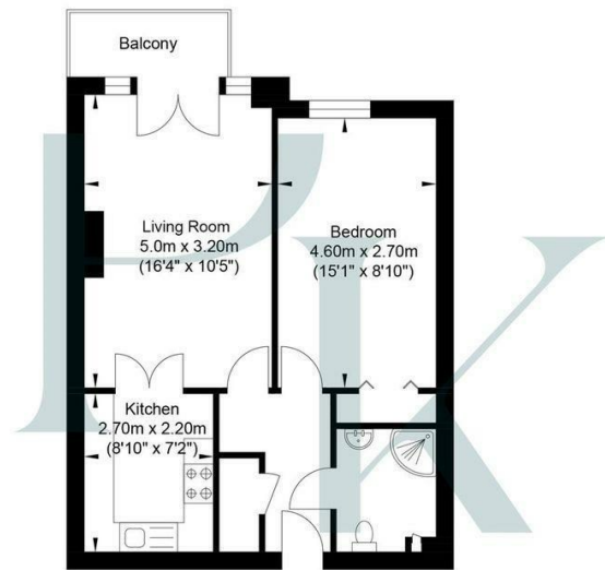
Second Floor Approximate Floor Area 491.69 sq ft (45.68 sq m)
