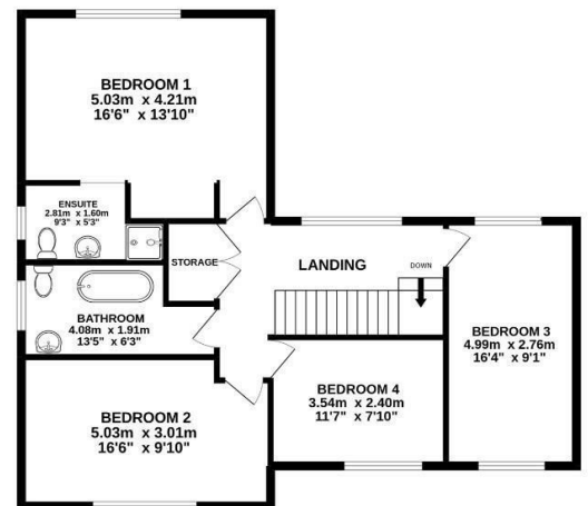
1ST FLOOR 80.5 sq.m. (866 sq.ft.) approx.
