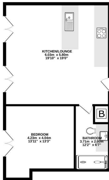
GROUND FLOOR 58.2 sq.m. (626 sq.ft.) approx.
