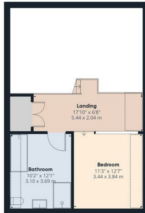
Floor 1
