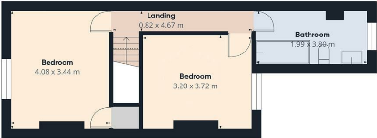
Floor 1
