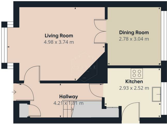
Floor 0 Building 1
