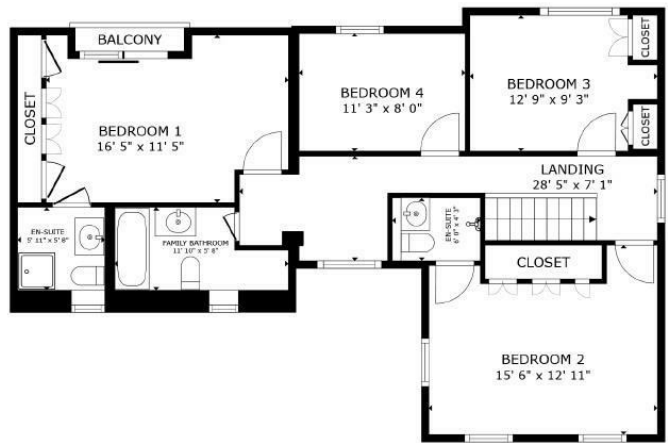
FLOOR 2
