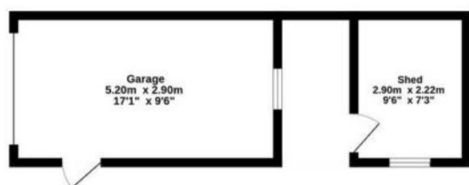
Garage 25.9 sq.m. (279 sq.ft.) approx.
