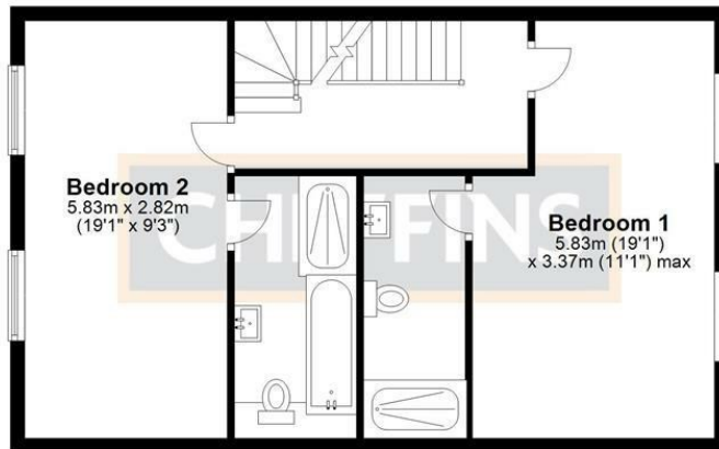
First Floor Approx. 56.0 sq. metres (602.6 sq. feet)
