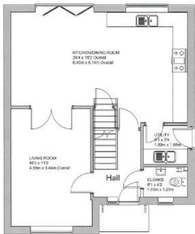
GROUND FLOOR APPROX. FLOOR AREA 677 SQ.FT. (63 SQ.M)
