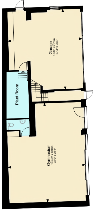
Coach House Ground Floor
