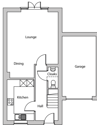
GROUND FLOOR
