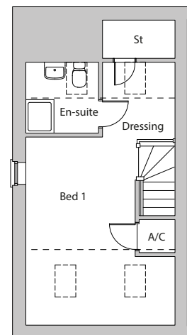
SECOND FLOOR
