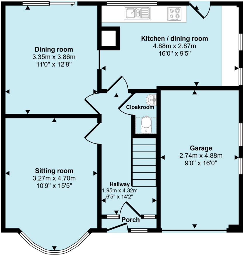
Ground Floor Approx 67 sq m / 721 sq ft
