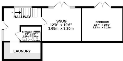
LOWER GROUND FLOOR 438 sq.ft. (40.7 sq.m.) approx.
