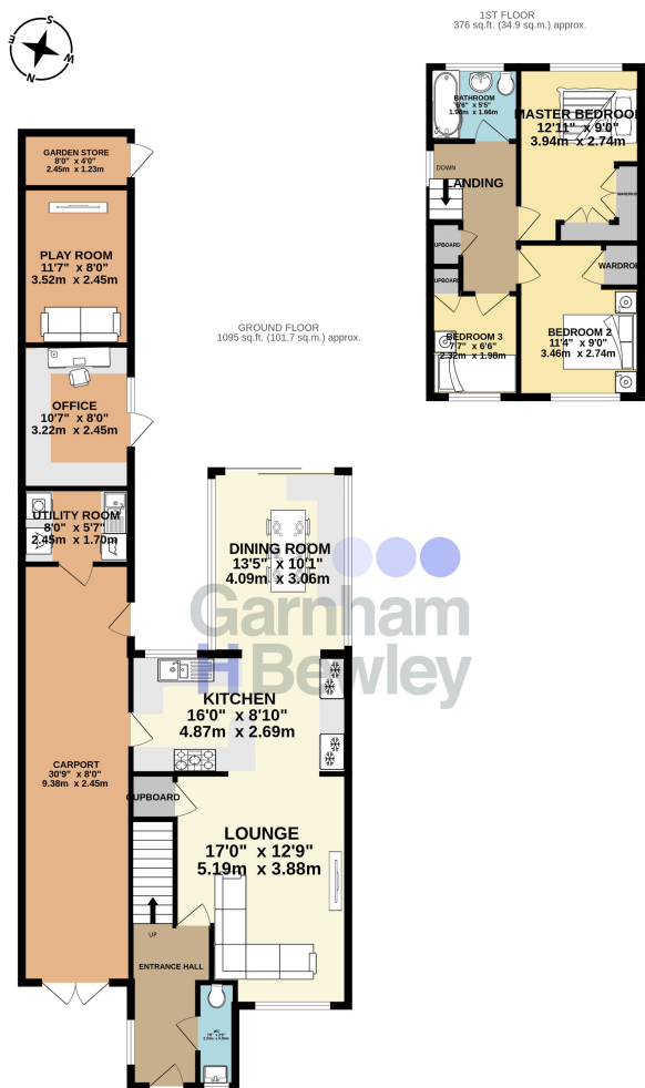
50 FOREST CLOSE - FLOORPLAN
