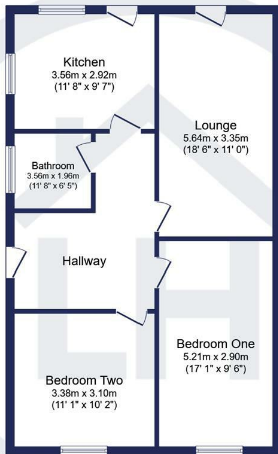
Floor Plan Floor area 71.7 sq.m. (772 sq.ft.)
