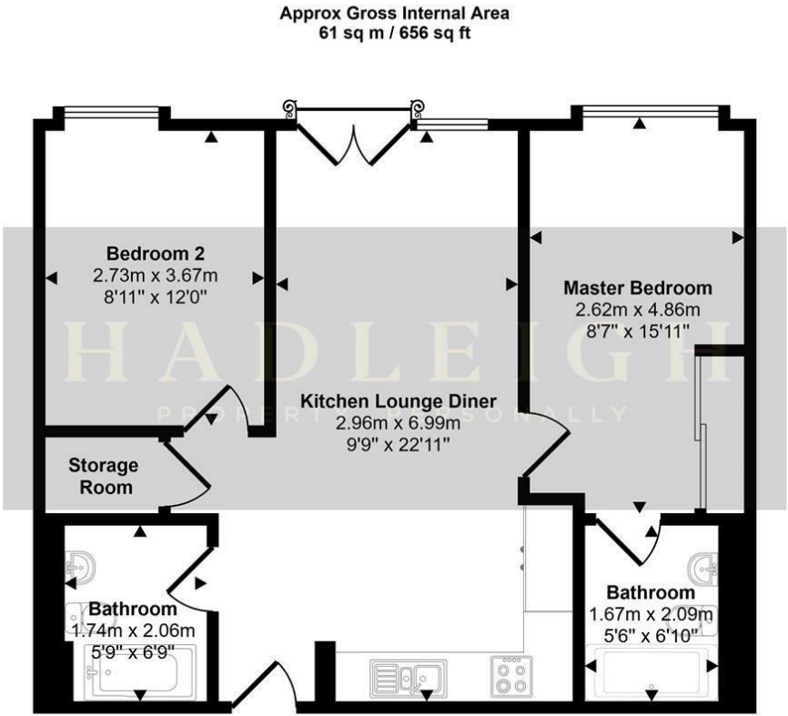
Floorplan
