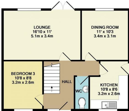
GROUND FLOOR APPROX. FLOOR AREA 732 SQ.FT. (68.0 SQ.M.)
