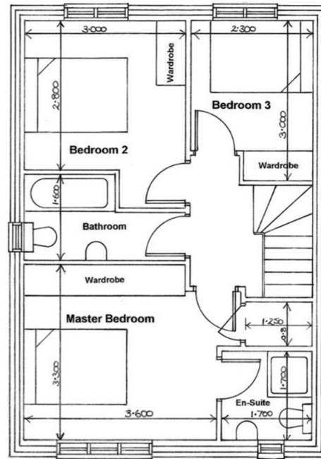
Plot 15 & 7 First Floor Layout Plan
