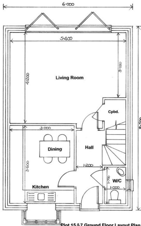
Plot 15 & 7 Ground Floor Layout Plan
