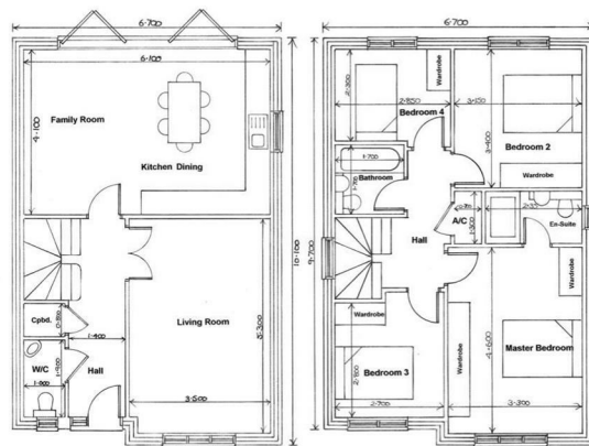
Plot 6 Ground Floor Layout Plan
