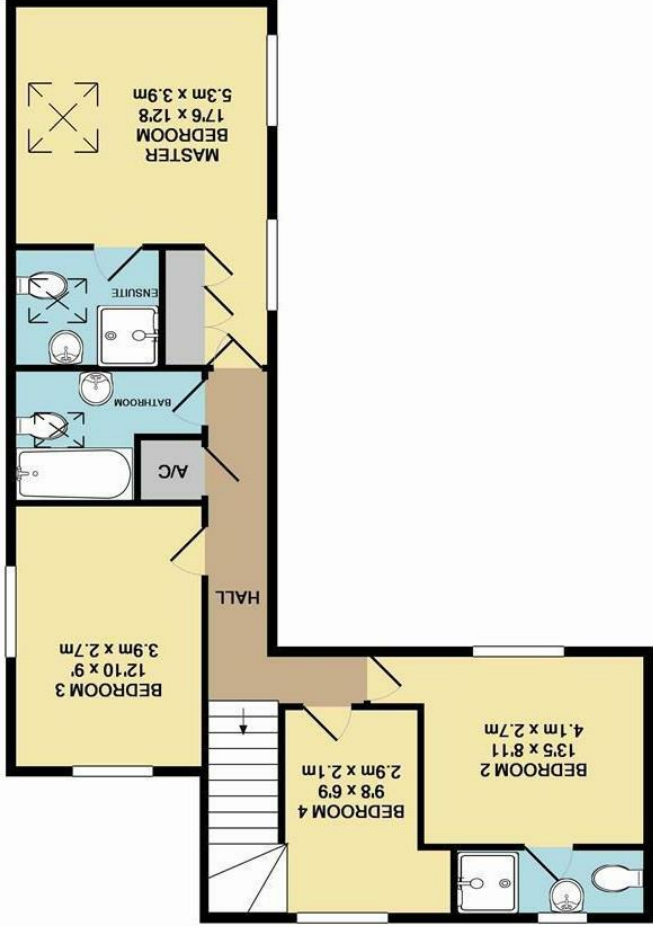
1ST FLOOR APPROX. FLOOR AREA 708 SQ.FT. (65.7 SQ.M.)
