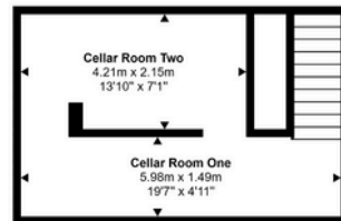
Cellar Approx 23 sq m / 244 sq ft
