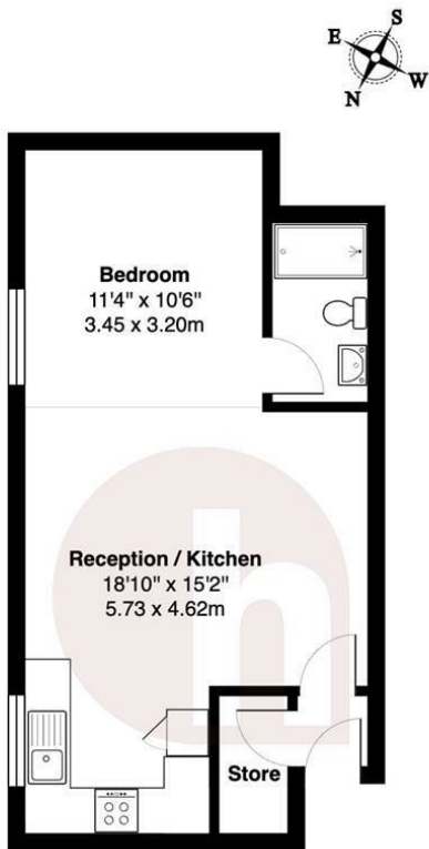
2nd Floor
