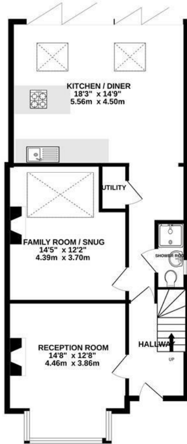
GROUND FLOOR 776 sq.ft. (72.1 sq.m.) approx.
