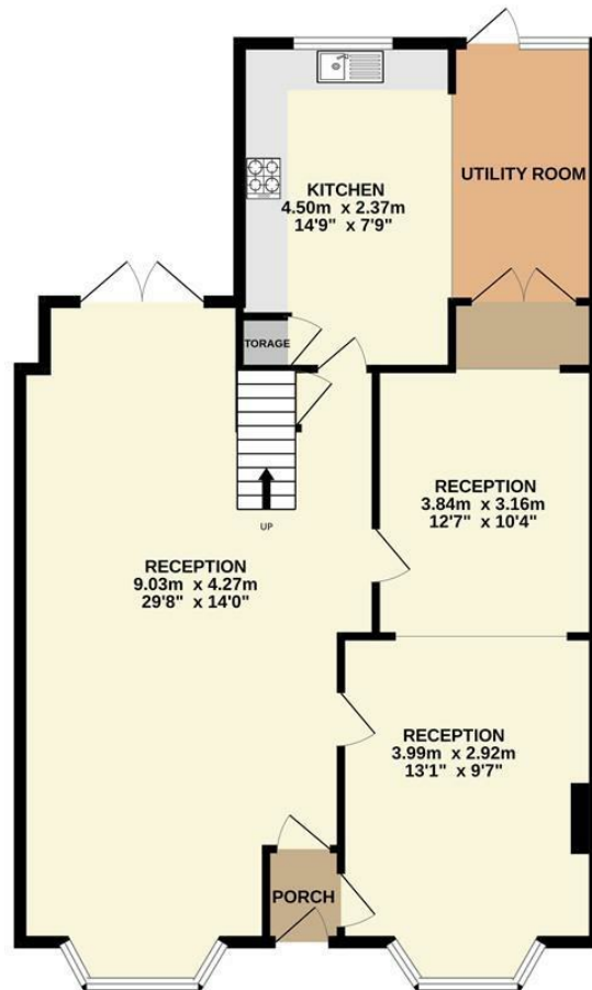
GROUND FLOOR 85.0 sq.m. (915 sq.ft.) approx.
