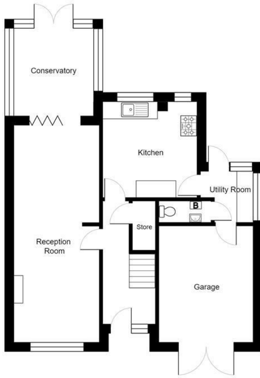
Ground Floor Area: approx 77.6 m 2 ... 835 ft 2
