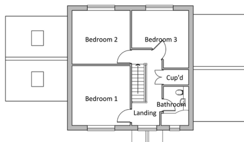
First Floor Layout 1:100
