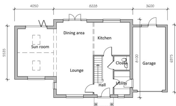
Ground Floor Layout 1:100
