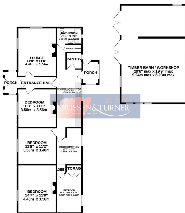
GROUND FLOOR 1712 sq.ft. (159.0 sq.m.) approx.
