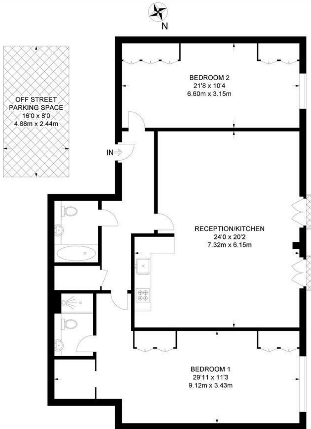
FIRST FLOOR
