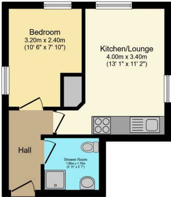
Floor Plan Floor area 26.2 m 2 (282 sq.ft.)
