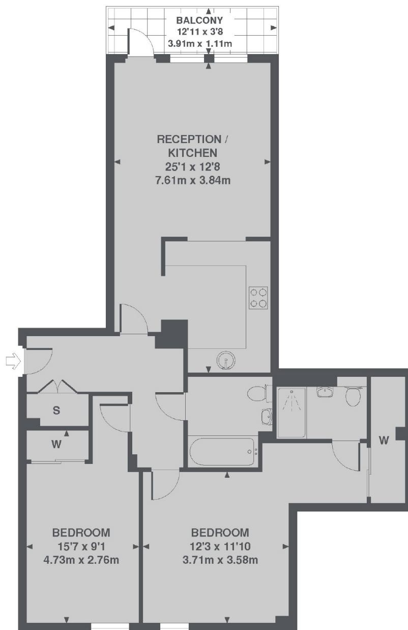
SECOND FLOOR
