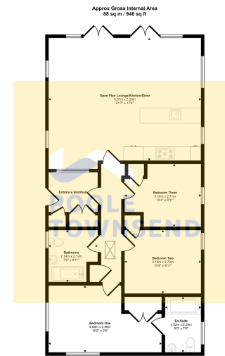
Floorplan
