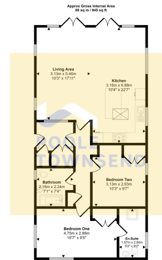
Floorplan
