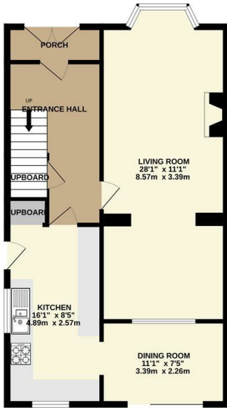
GROUND FLOOR 657 sq.ft. (61.0 sq.m.) approx.
