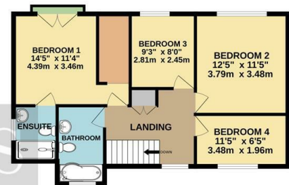
1ST FLOOR 648 sq.ft. (60.2 sq.m.) approx.
